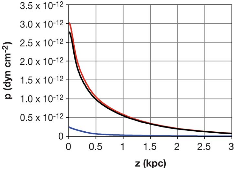
Figure 2 Comparison of the total ( red ) and volume average thermal ( blue ) pressure distributions, and their difference ( black ) interpreted as the nonthermal pressure. In this case, the total is taken from the weight distribution of the ISM. The thermal pressure neglects any contribution from the hot component.
