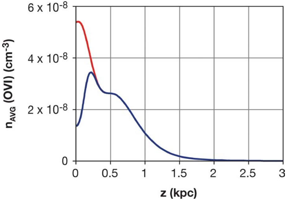
Figure 6 The distribution of average interstellar density of OVI, assuming that all SNe occur in the total average density (blue) or diffuse density (red). The observed midplane value is about 1.7 \times 10^{-8} \text{ cm}^{-3} .
