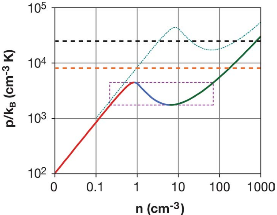
Figure 7 The Two-Phase Medium thermal pressure versus density curve is shown in the red-blue-green curve. The red segment is the thermally stable warm component, the green the corresponding stable cold component, and the blue the thermally unstable regime. The black dashed line is the total midplane pressure, the orange dashed line represents the magnetic pressure, the dashed aqua line shows how the p(n) curve shifts when the heating rate is raised considerably, and the dashed purple rectangle outlines the regime of essentially zero bulk modulus.
