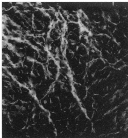
Fig. 1. An image of the force chains in a granular medium as viewed between two crossed circular polarizers. The particles, 3-mm Pyrex spheres, are surrounded by an index-matching fluid, a mixture of glycerol and water. The beads are placed in a box with sides 70 mm by 70 mm by 40 mm; the image size is 40 mm by 42 mm. A 200-N force is exerted on a piston that covers the top surface. The stressed beads can be seen as bright regions (the brightness is due to their stress-induced birefringence).
