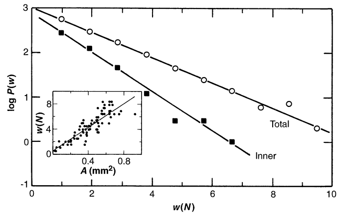
Fig. 2. The distribution of forces P(w) versus force w measured at the bottom of a cylindrical container 90 mm in diameter filled to a height of 75 mm with glass spheres having a radius of 3.5 mm. The bottom of the container was lined with carbon paper, and a force of 310 N was applied to the top surface. The inset shows that the area of a mark on the carbon paper is proportional to the force exerted by the individual bead. In the main panel, the circles show data taken from the entire base of the container; the squares show the data taken only from the region close to the axis (within half of the cylinder's radius). The data are the cumulative results of five separate trials. The lines are exponential fits to the data: P(w) = Ce^{-Aw} with A = 0.64 \text{ N}^{-1} and C = 988 for the total and A = 1.02 \text{ N}^{-1} and C = 736 for the inner region.
