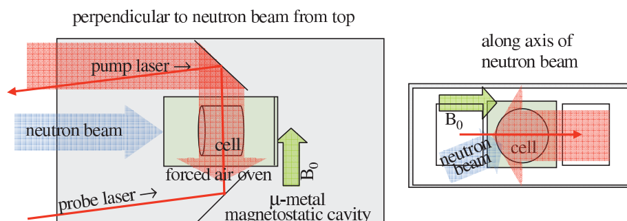
Figure 1. The spin-exchange optical pumping setup used for this experiment. One pump laser was used which counter propagated with the probe laser.
