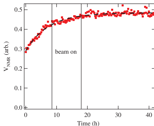
Figure 5. The measured relative ^3\text{He} polarization vs. time for the Roadrunner cell, a double chamber cell, via NMR free induction decay. During the time labelled "beam on" the spin filter portion of the cell was exposed to the flux of the neutron beam while continuing to polarize the cell via the spin-exchange chamber which was outside of the neutron beam. The observed ^3\text{He} polarization was not affected by the absorbed neutron flux in the spin filter chamber.
