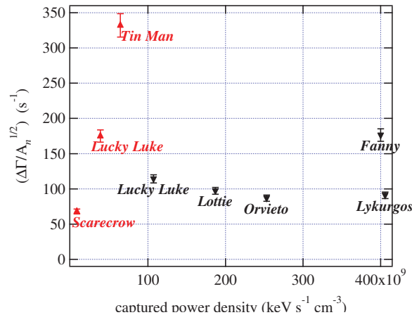
Figure 6. The measured change in alkali-metal relaxation verses captured power density for the cells from the PB1B experiment [12] (black downward triangles) and the sealed cells from this work (red upward triangle). All of the values of \Delta\Gamma have been normalized to the square root of the normalized absorbed neutron flux, where the normal neutron flux (i.e. flux=1) was taken as the full flux of the tomography beam line used in this work.
