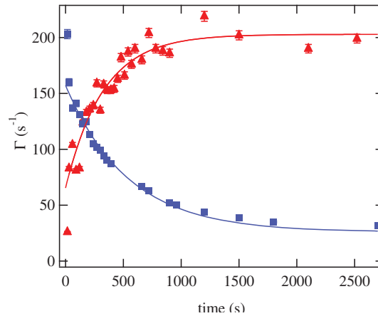
Figure 2. A sample of the measured alkali-metal relaxation rates, \Gamma , as a function of time after the beam was opened, red triangles, or closed, blue squares, for the cell Tin Man.
