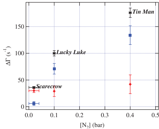
Figure 3. The measured alkali-metal relaxation versus [\text{N}_2] for the sealed cells. Black bow-ties are the total change in measured alkali-metal relaxation, blue squares are the deduced slow portion, and red diamonds are the deduced fast portion. The x-axis error bars for the Scarecrow cell are included because the value of [\text{N}_2] for this cell was estimated from its optical pumping properties and has an uncertainty of \pm 0.02 bar.
