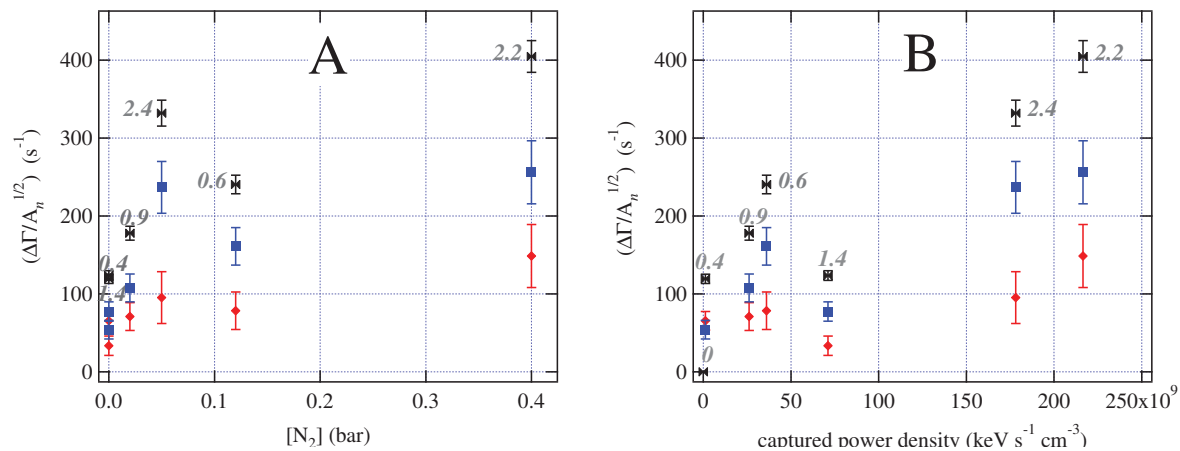
Figure 4. The measured alkali-metal relaxation versus [\text{N}_2] (graph A) and captured power density (graph B) for the valved cell with different gas fillings. In both graphs the values of \Delta\Gamma have been normalized by A_n^{1/2} to account for the flux dependence shown in Ref. [12]. Black bow-ties are the total change in alkali-metal relaxation, blue squares are the deduced slow portion, and red diamonds are the deduced fast portion. The numbers labelling the markers denote the ^3\text{He} pressure of the cell for the particular cell filling as given in Table 1.
